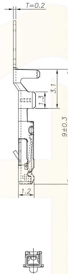
SECTION C-C
