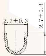
SECTION C-C
